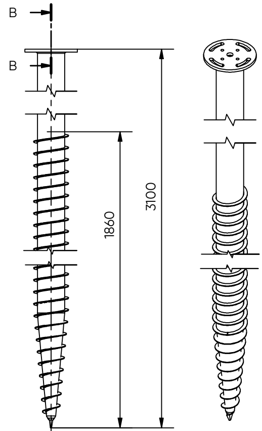
Side view ( 1 : 16 )
