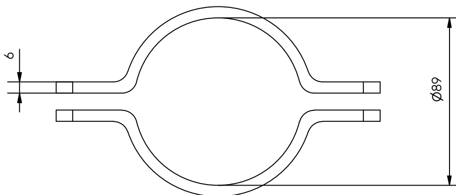
3D view (1:3)
