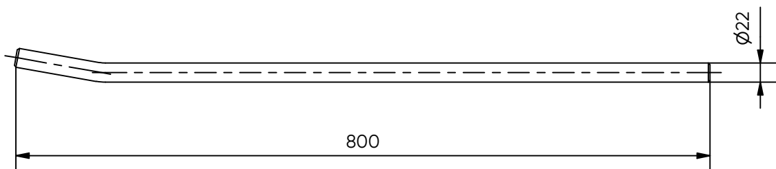
Side view (1 : 6)
