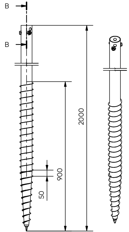
Side view ( 1 : 16 )
