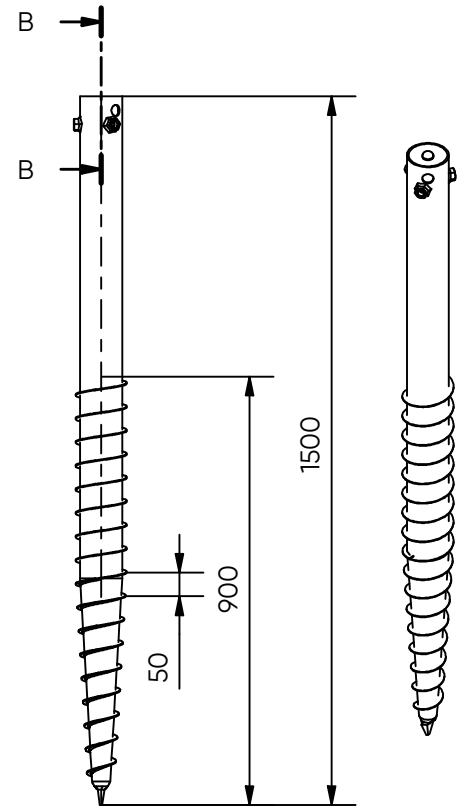
3D view (1 : 16)
