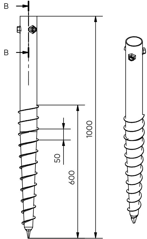
Side view ( 1 : 10 )
