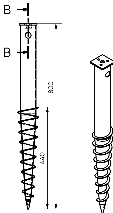
Side View (1 : 8)
