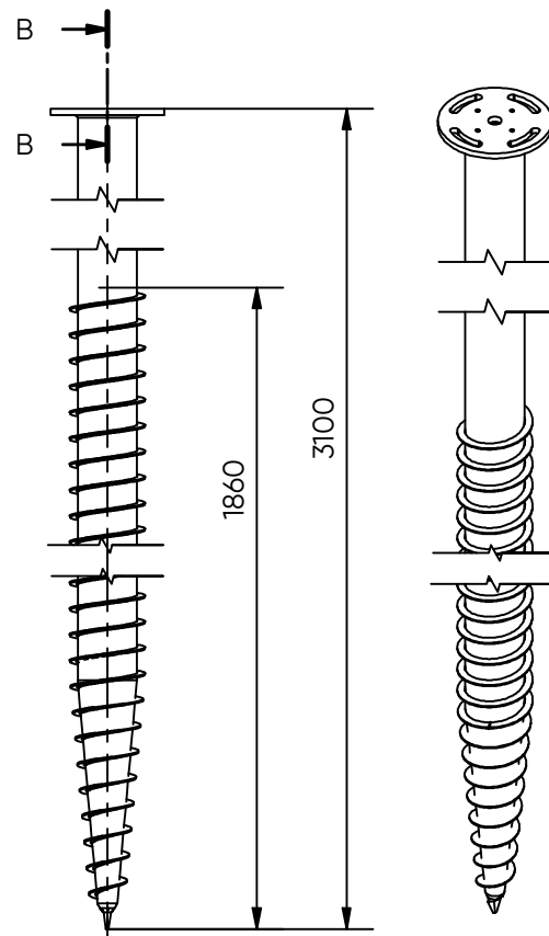
Side view ( 1 : 16 )
