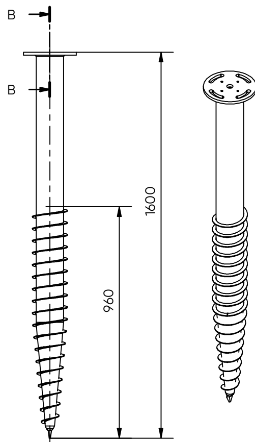
Side view ( 1 : 16 )
